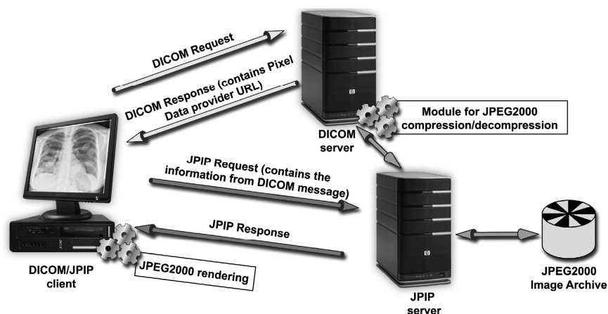
Fig. 9. Standard DICOM JPIP Provider JPIP Repository Architecture – the DICOM JPIP Pixel Data Provider service where all the images are stored at JPIP server-side application; DICOM server stores and requests images from JPIP server
