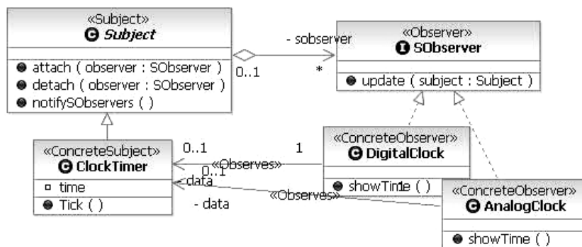
Fig. 4. The result of the transformation to Java target platform of the model from Fig. 3 in accord with the instance suggestion and specification
