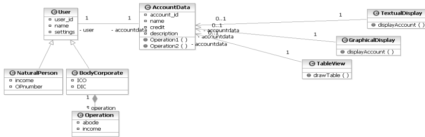
Fig. 10. Example of starting UML model before the application of patterns
