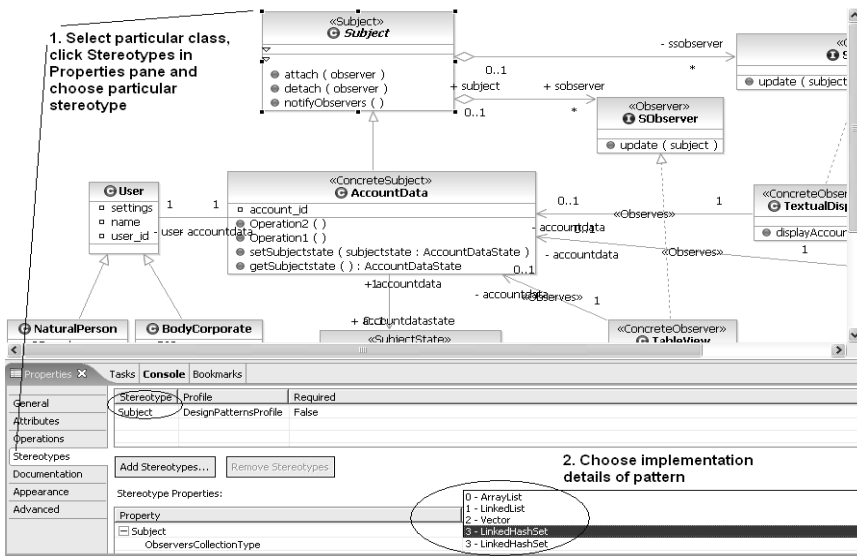
Fig. 16. Choosing of implementation details of pattern instances
