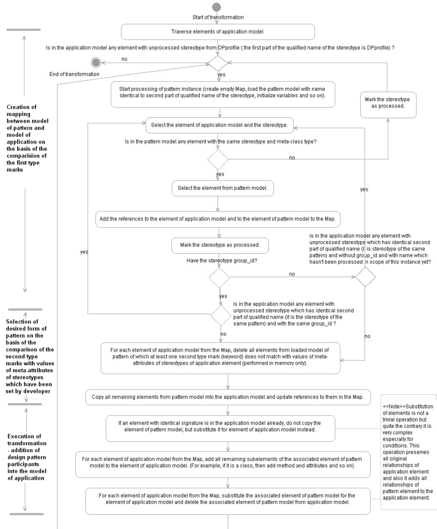
Fig. 8. Principles of tool functioning - tool under the hood.
