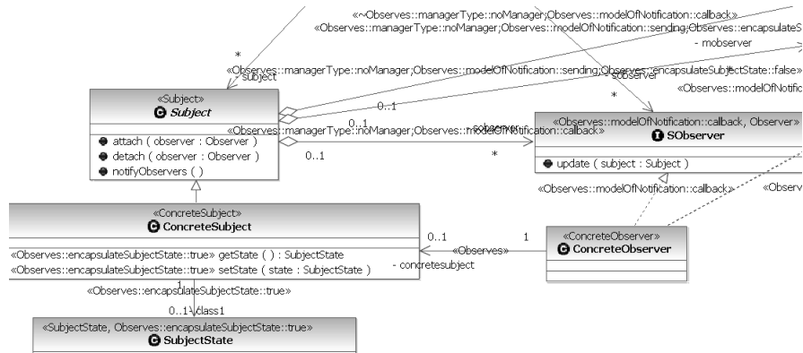
Fig. 7. Sample section of Observer pattern model by which the transformation is driven
