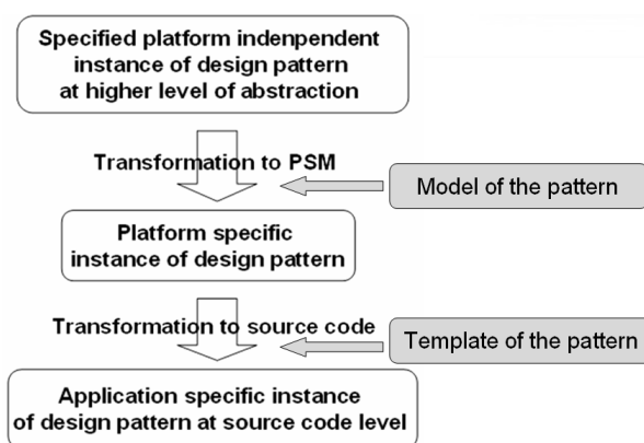
Fig. 2. Proposal of design pattern instantiation process
