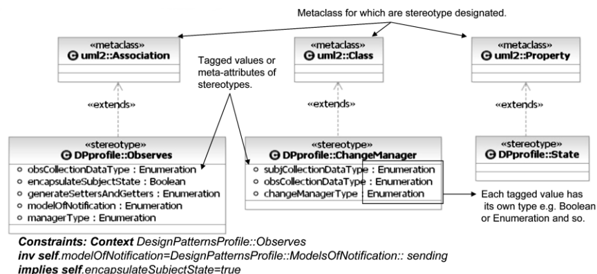
Fig. 6. The snippet of UML profile with some elements for Observer pattern
