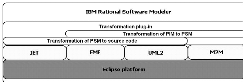
Fig. 18. The architecture of the implemented tool
