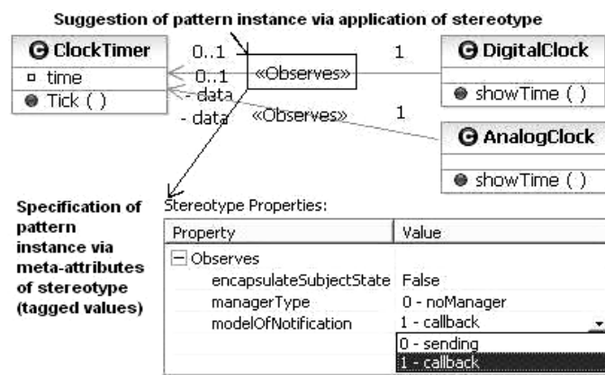
Fig. 3. Example of an application of the Observer pattern to a model. It represents a specified platform independent instance and thus the most abstract form of the Observer pattern instance
