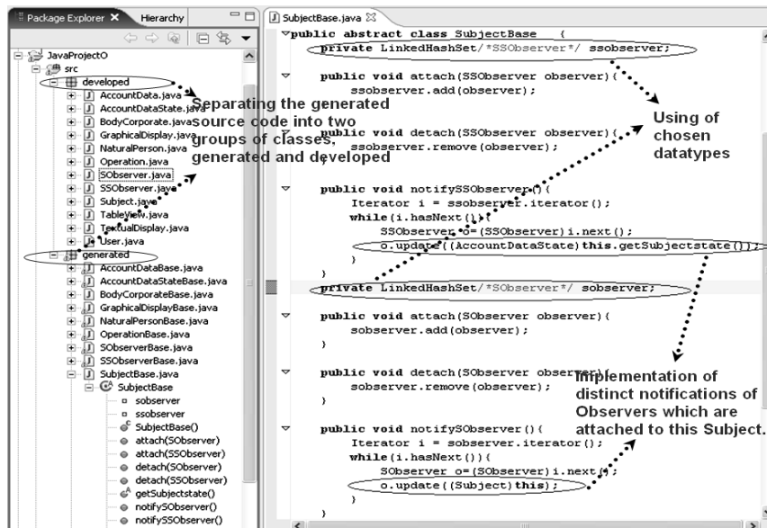
Fig. 17. The snippet of resulting source code of transformation of model from Fig. 16 to Java source code
