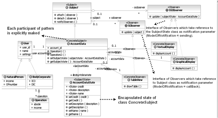
Fig. 15. The resulting model of transformation of model from Fig. 13
