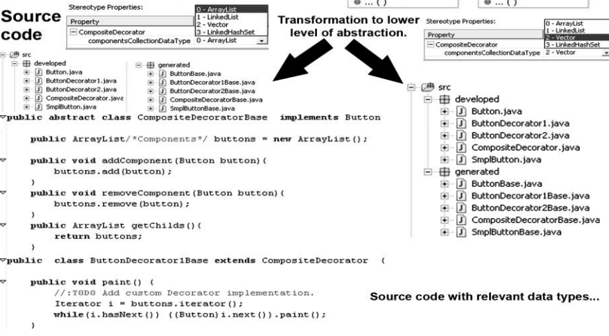
Fig. 5. An overall illustration of the pattern instantiation process
