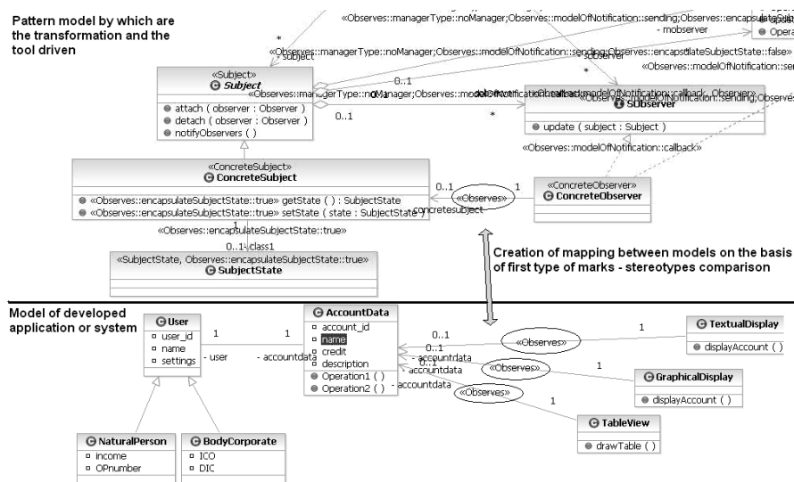
Fig. 12. Creation of mapping between model of developing application or system and pattern model by which the tool and the transformation are driven
