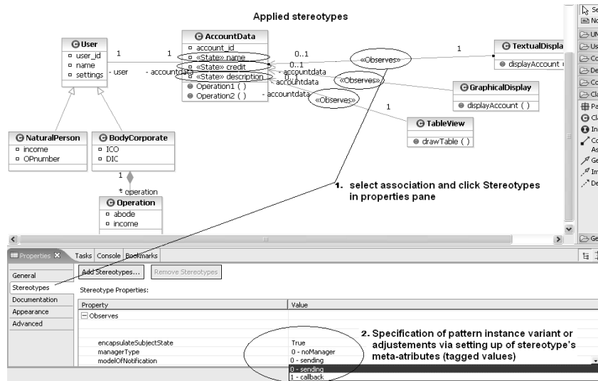
Fig. 13. Setting up of values of stereotype meta-attributes
