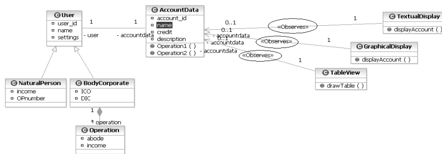
Fig. 11. The resulting model after pattern instances suggestion
